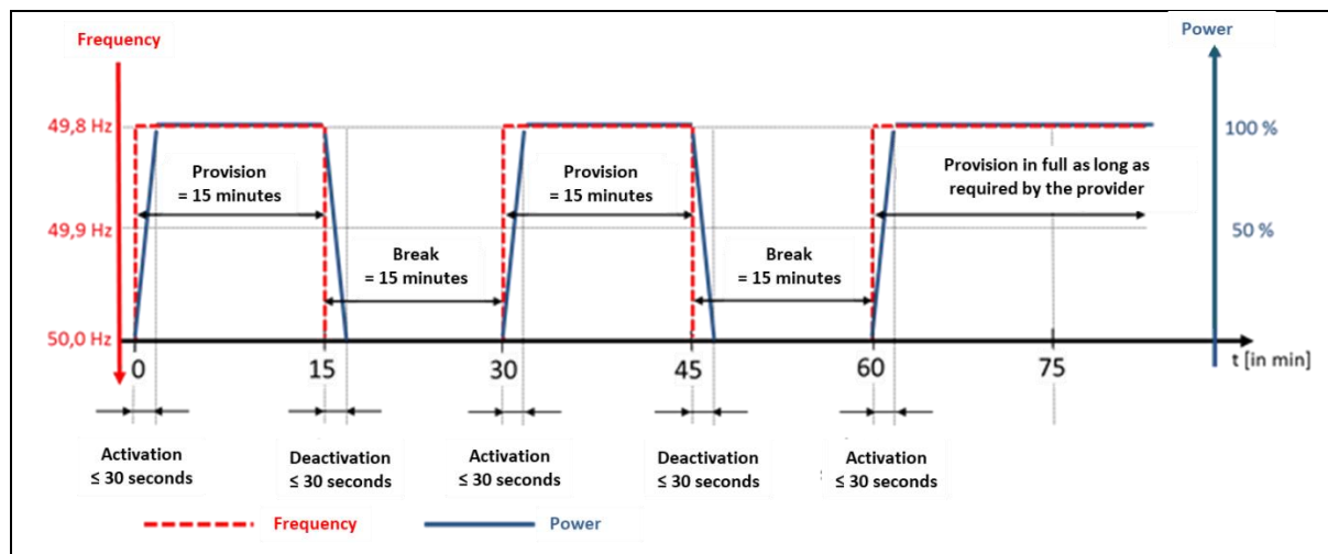
Figure 11: Variant 1 of the verification of the usable energy capacity (FCR)
