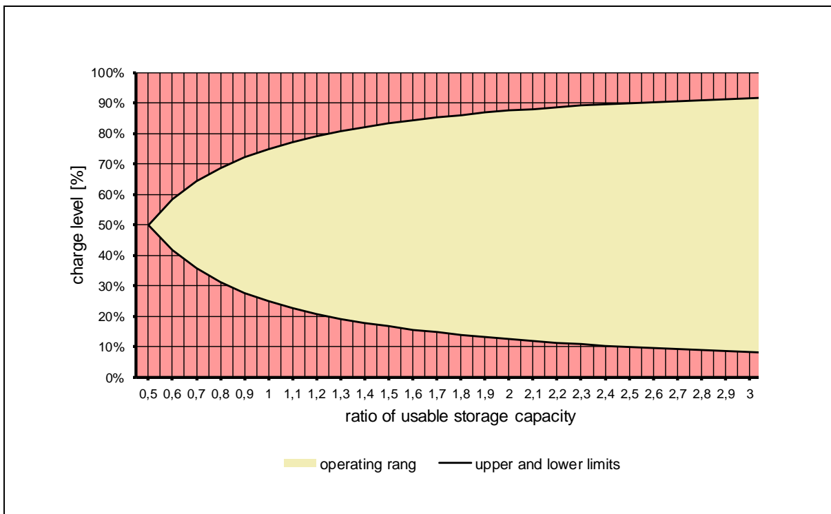
Figure 17: Permissible operating range for FCR units and FCR groups with limited energy storage
