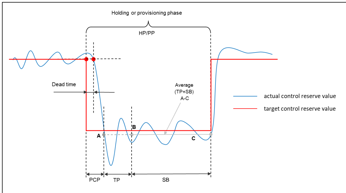
Figure 4: Schematic representation of an FCR operating test
