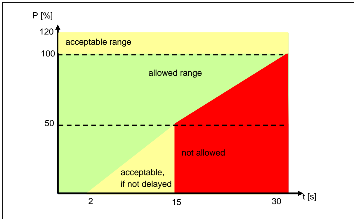
Figure 14: Artificial deceleration FCR (visualization without consideration of fluctuation tolerances)
