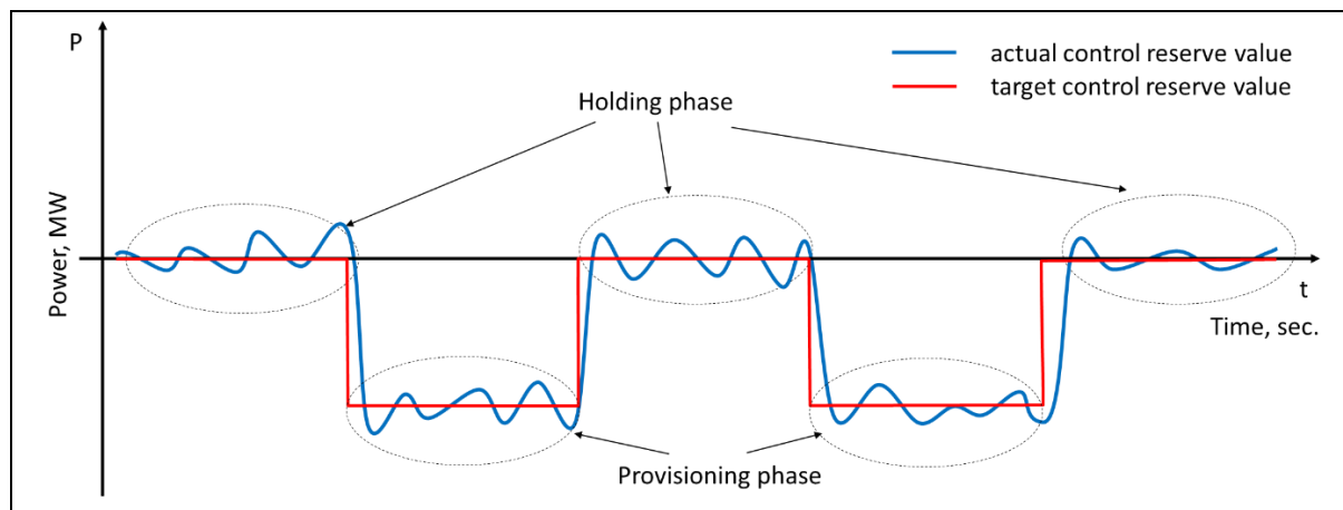
Figure 3: Evaluation of the operating test through combination of the raw data
