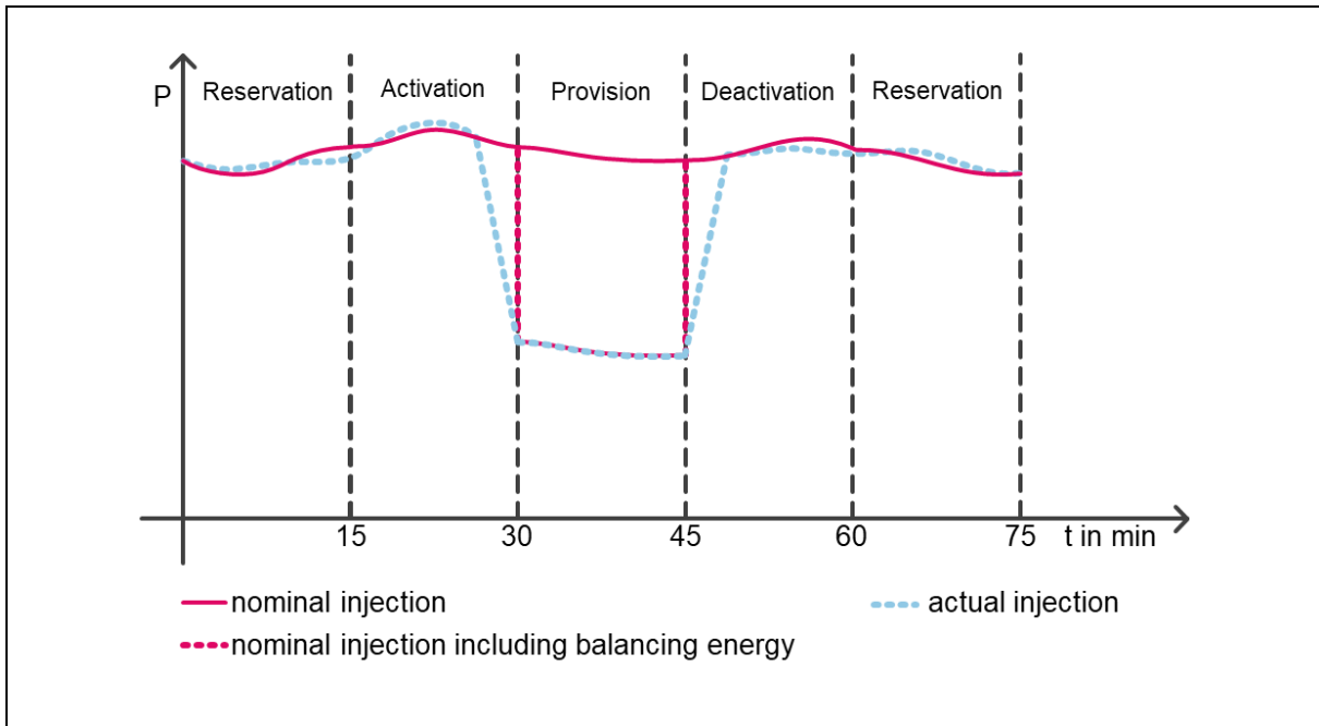
Figure 13: Verification procedure of the "nominal injection" method using the example of mFRR
